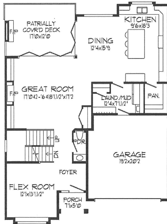
MAIN FLOOR 1,297 SQ FT
