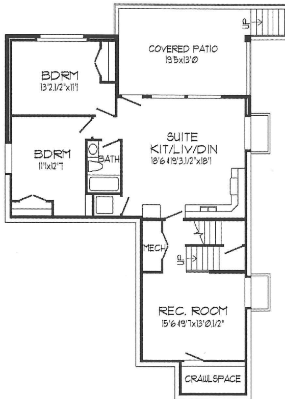
BASEMENT SUITE FLOOR 1,309 SQ FT
