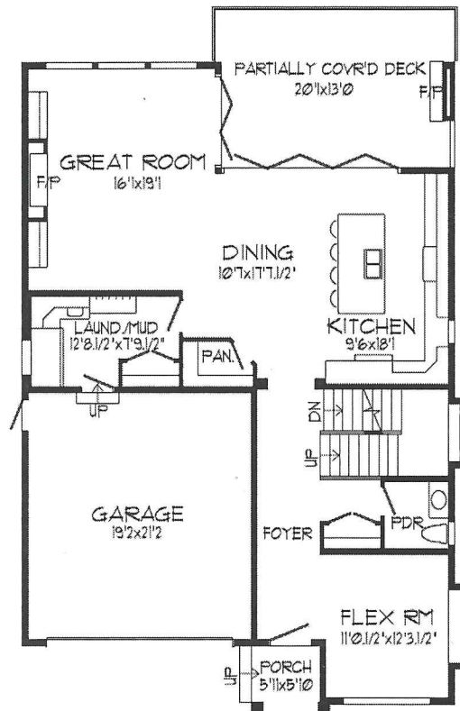
MAIN FLOOR 1,320 SQ FT
